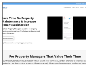
Laravel Saas
