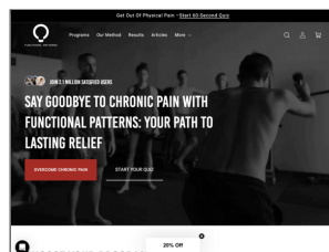
Shopify + Laravel
